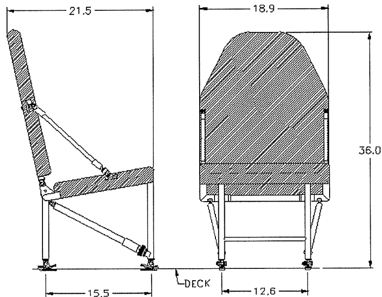
Figure 1.1.1 Basic Seat Dimensions
