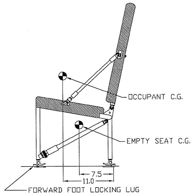
Figure 1.4.2 Seat Center of Gravity
