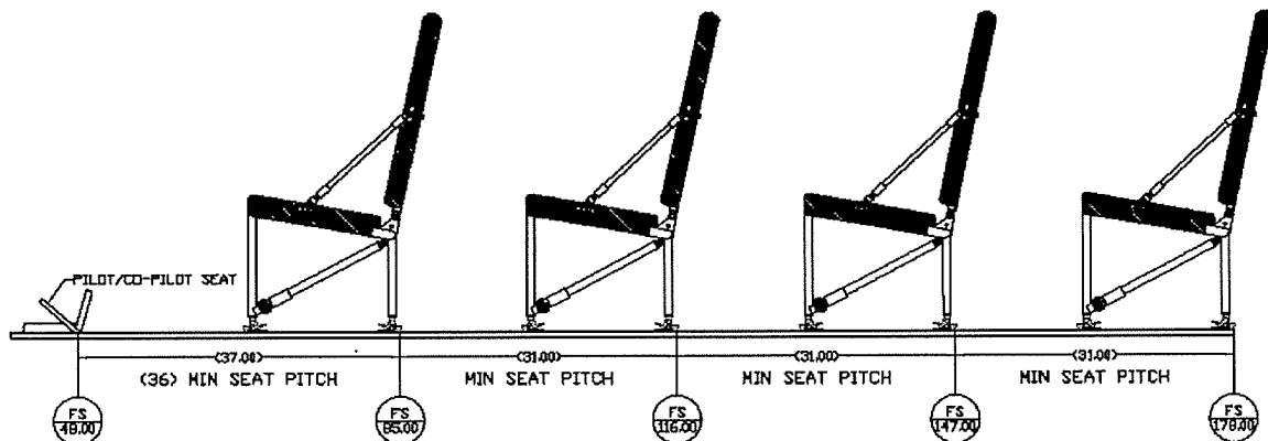
Figure 1.4.1 Approved Seat Locations and Spacing Requirements
