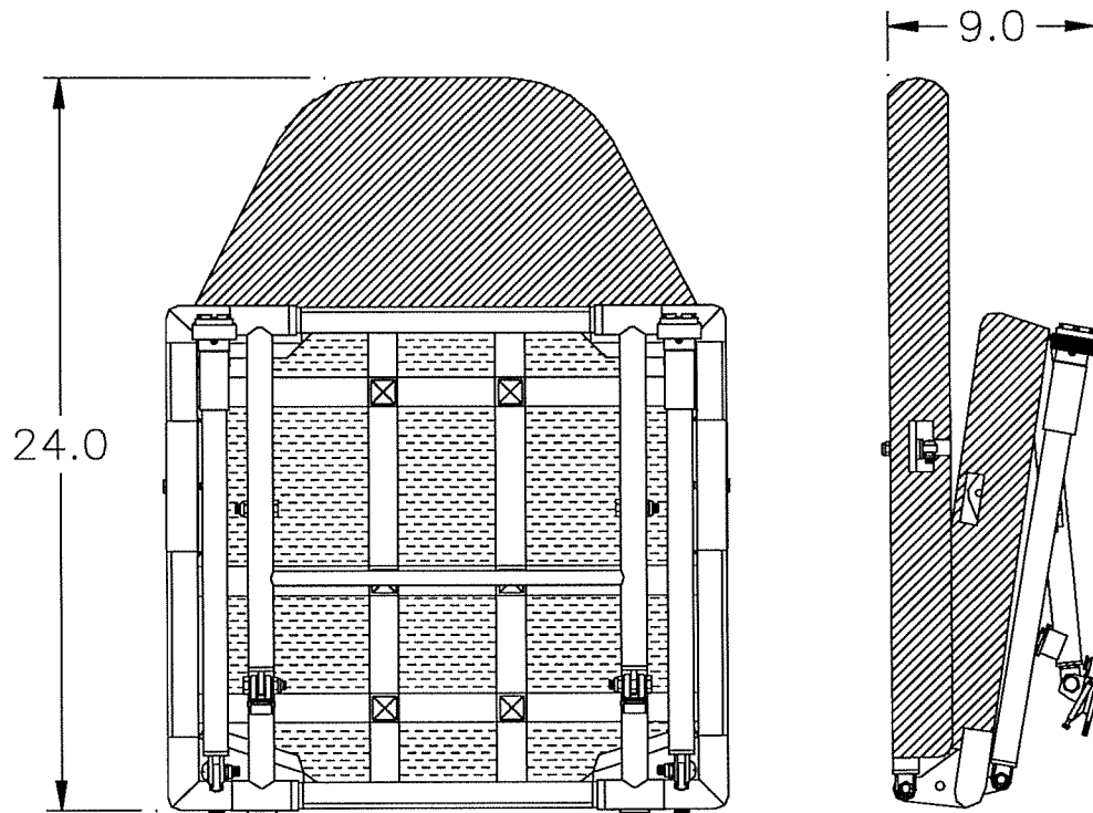
Figure 1.1.2 Folded Seat Dimensions
